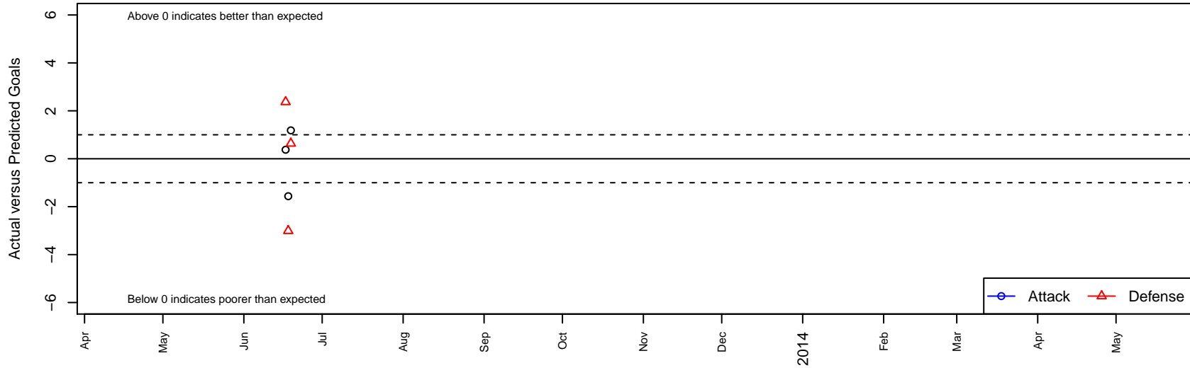
Hawaii LJSA 00 Chelsea B99 Dots are actual minus expected GF (blue circles) and GA (red triangles). Blue line is smoothed change in attack strength. Red is smoothed change in defense strength.
